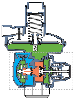
Figure 1: Front View Schematic
